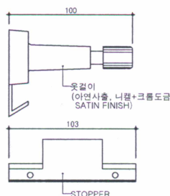
돛걸이/STOPPER SCALE : 1/3
